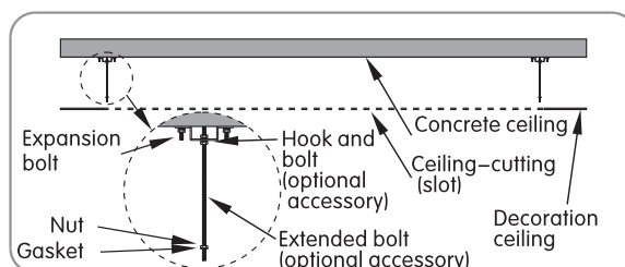
Diagram 9 Use hook for installation to high ceiling
