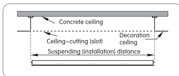
Diagram 7 Use hook for installation to high ceiling
