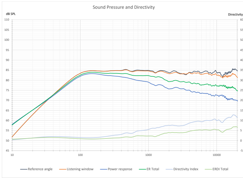
Horizontal Directivity
